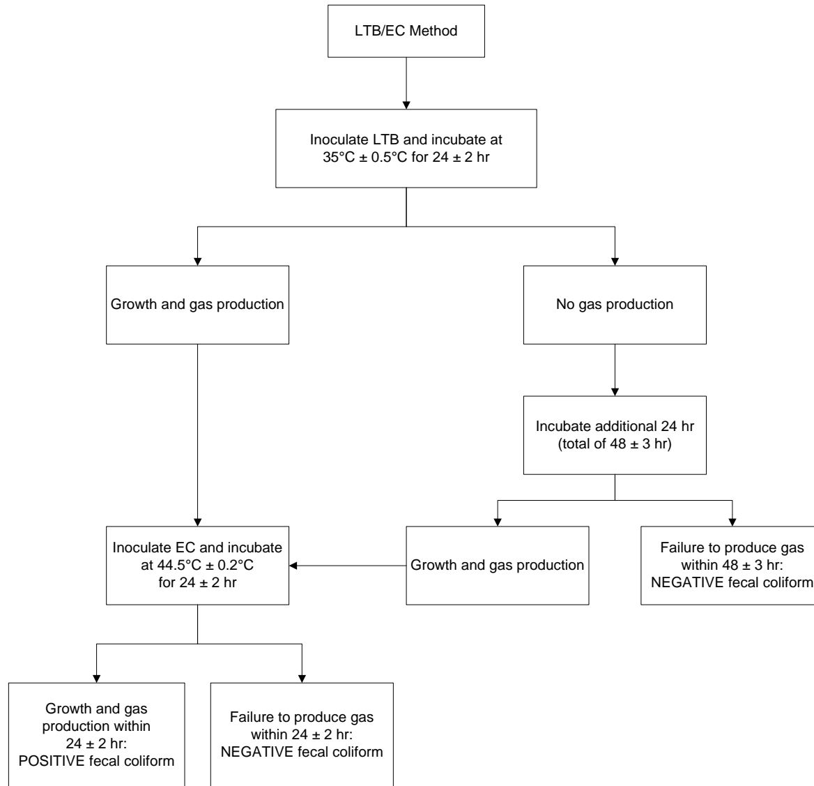
FIGURE 1. MULTIPLE TUBE FERMENTATION PROCEDURE
